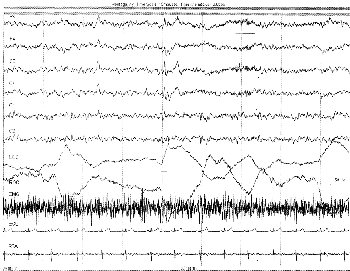
Figure NR5. Hypnogram and PSG tracing from 25-year-old female with INM. A section of stage 1 sleep with spindling at sleep onset contains both medium fast and rapid eye movements in the same eye movement burst. Legend as in Figure NR4.
