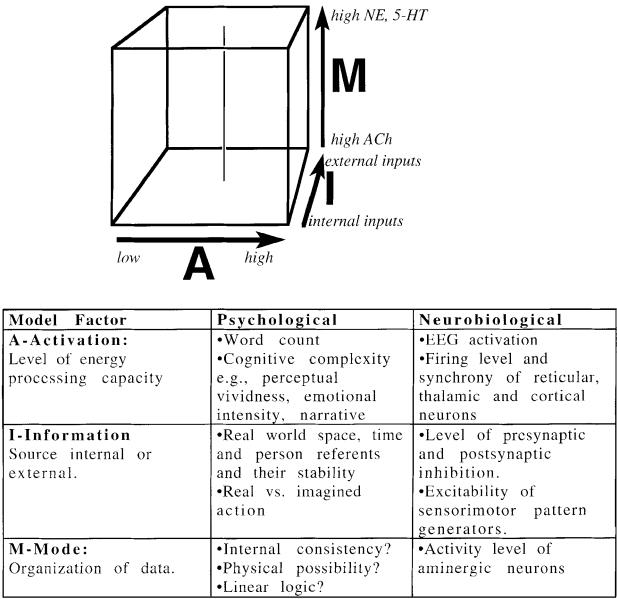
Figure 1. The Activation-Input Source-Neuromodulation model (AIM). Illustration of three dimensional state space and the psychological neurobiological correlates of each dimension. See section 4 and also Hobson (1990; 1992a; 1997a).
