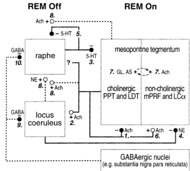
Figure 4. Additional synaptic details of the revised reciprocal interaction model shown in Figure 3B derived from data reported (solid lines) and hypothesized relationships suggested (dotted lines) in recent experimental studies (numbered on Figure and below). See text for discussion of these findings. Additional synaptic details can be superimposed on the revised reciprocal interaction model without altering the basic effects of aminergic and cholinergic influences on the REM sleep cycle. Excitatory cholinergic-non-cholinergic interactions utilizing Ach and the excitatory amino acid transmitters enhance firing of REM-on cells (6, 7) while inhibitory noradrenergic (4), serotonergic (3), and autoreceptor cholinergic (1) interactions suppress REM-on cells. Cholinergic effects upon aminergic neurons are both excitatory (2), as hypothesized in the original reciprocal interaction model and may also operate via presynaptic influences on noradrenergic-serotonergic as well as serotonergic-serotonergic circuits (8). GABAergic influences (9, 10) as well as other neurotransmitters such as adenosine and nitric oxide (see text) may contribute to the modulation of these interactions. Abbreviations: open circles, excitatory postsynaptic potentials; closed circles, inhibitory postsynaptic potentials; mPRF, medial pontine reticular formation; PPT, pedunculopontine tegmental nucleus; LDT, laterodorsal tegmental nucleus; LCα, peri-locus coeruleus α; 5HT, serotonin; NE, norepinephrine; Ach, acetylcholine; GL, glutamate; AS, aspartate; GABA, gamma-aminobutyric acid. References: (1) Baghdoyan et al. 1997; El Manseri et al. 1990; Kodama & Honda 1996; Leonard & Llinas 1990, 1994; Luebke et al. 1993; Roth et al. 1996; Sakai & Koyama 1996; Sakai et al. 1990. (2) Egan & North 1985; 1986b. (3) Horner et al. 1997; Leonard & Llinas 1994; Luebke et al. 1992; Thakkar et al. 1997. (4) Sakai & Koyama 1996. (5) Portas et al. 1996. (6) Sakai & Koyama 1996; Sakai & Onoe 1997; Vanni-Mercier et al. 1989; Yamamoto et al. 1990a; 1990b. (7) Greene & McCarley 1990; Leonard & Llinas 1994; Sakai & Koyama 1996. (8) Li et al. 1997. (9) Nitz & Siegel 1997; Datta 1997b; Datta et al. 1991. (10) Porkka-Heiskanen et al. 1997a (from Hobson et al. 1998b).
