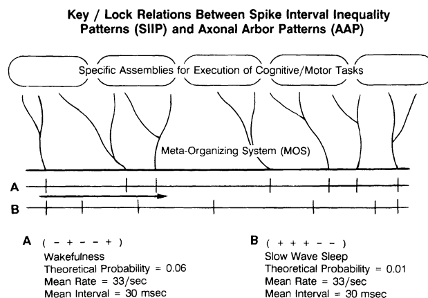
Figure 1 (Marczyński). Key/Lock relations between Spike Interval Inequality Patterns (SIIP) and Axonal Arbor Patterns (AAP).
